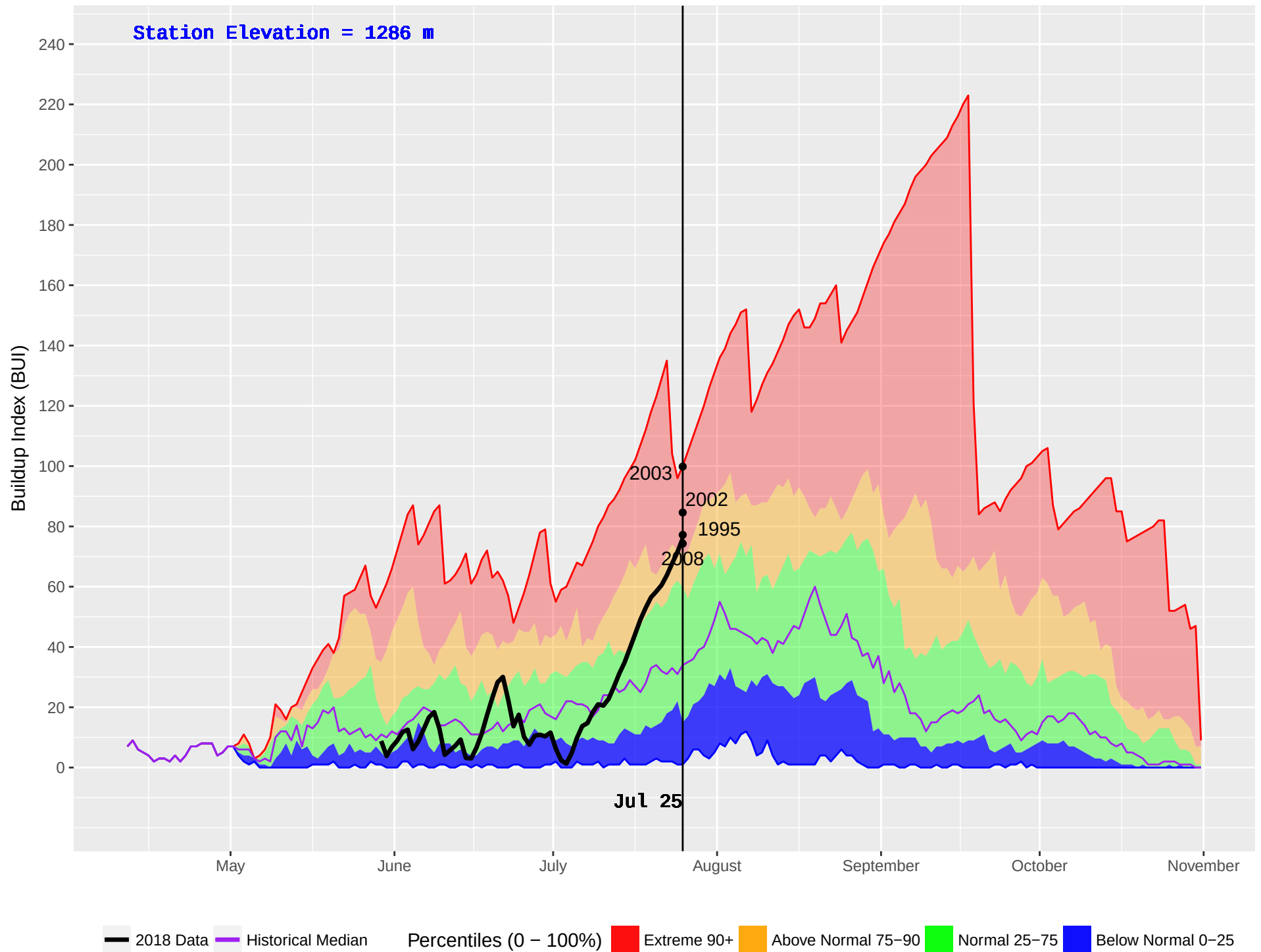
CURWEN CREEK (352) : Historical (1979–2016) and Current (2018) Noon Buildup Index (BUI)
