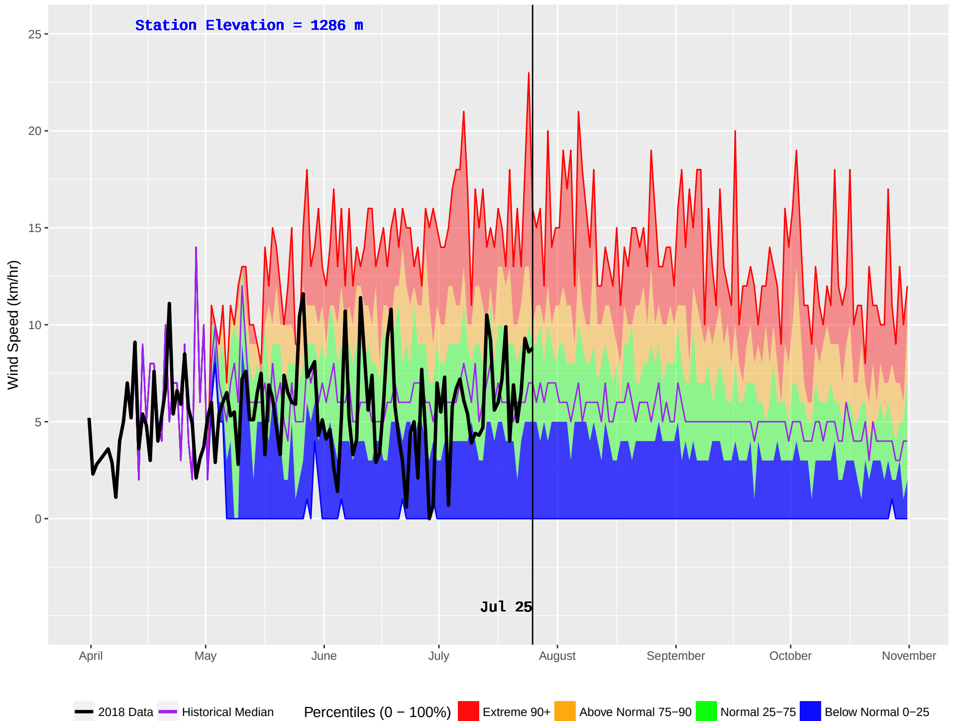
CURWEN CREEK (352) : Historical (1979–2016) and Current (2018) Noon Wind Speed
